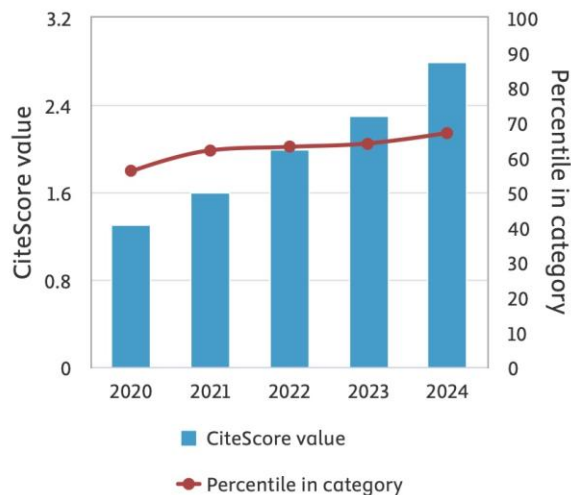
CiteScore trend
